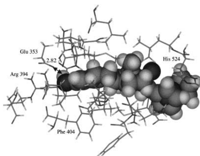
Figure 4. 17 \alpha -ruthenocenylmethylestradiol ( 7 ) in the hER \alpha cavity. The hormone 7 is represented as a space-filling model and the amino acids as rods. The amino acid His524 is clearly visible on the right of the cavity. Note the steric hindrance between the -\text{CH}_2(\eta^5\text{-C}_5\text{H}_5)\text{RuCp} group and the receptor residues neighboring His524.
