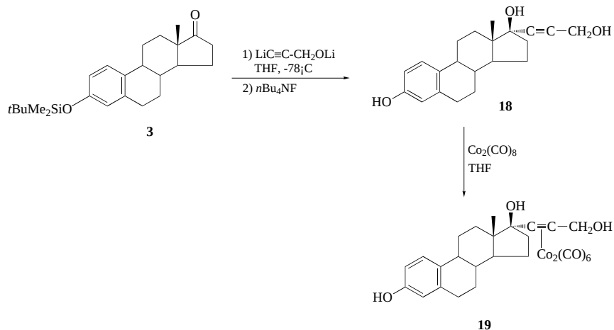
Scheme 6. Synthesis of cobalt complex 19 .
