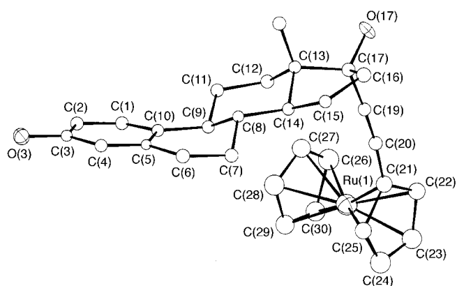
Figure 1. X-ray structure of 5 .
