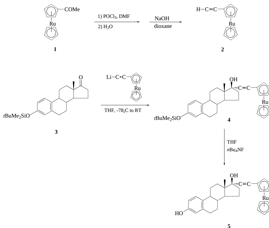
Scheme 1. Synthesis of 17\alpha -(ruthenocenylolethynyl)estra-1,3,5(10)-trien-3,17 \beta -diol ( 5 ).
