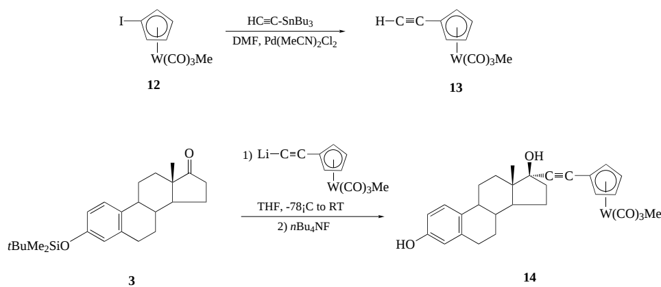
Scheme 4. Synthesis of tungsten complex 14 .
