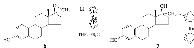
Scheme 2. Synthesis of 17\alpha -(ruthenocenylmethyl)estra-1,3,5(10)-trien-3,17 \beta -diol ( 7 ).
