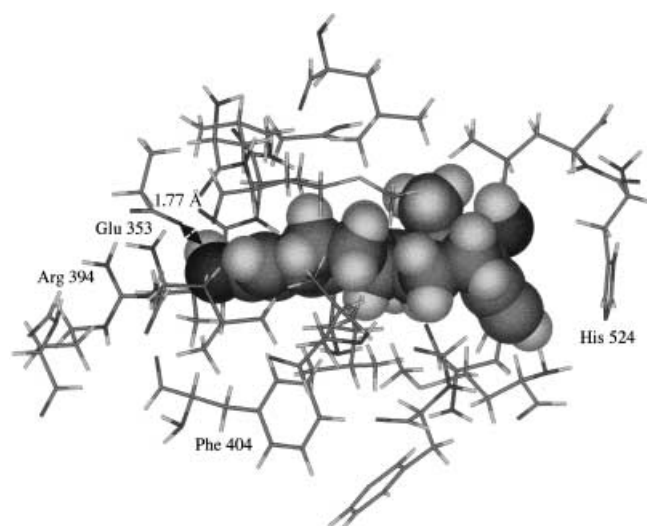
Figure 5. 17 \alpha -ethynylestradiol in the hER \alpha cavity. The hormone is represented as a space-filling model and the amino acid as rods. The amino acid His524 is clearly visible on the right hand of the cavity. It can be seen here that the ethynyl group at the 17 \alpha position does not present any steric constraint at this level, near to the narrow hydrophobic channel.
