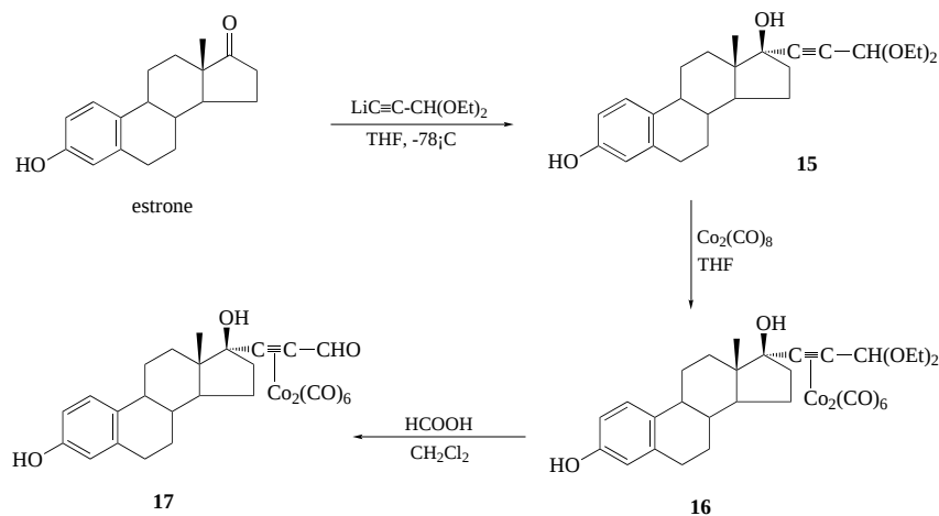
Scheme 5. Synthesis of cobalt complex 17 .
