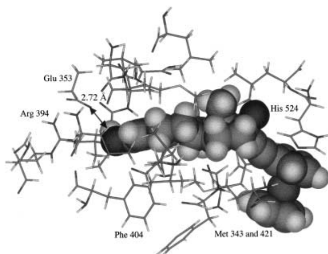
Figure 3. 17 \alpha -ruthenocenylethynylestradiol ( 5 ) in the hER \alpha cavity. The bioligand 5 is represented as a space-filling model and the amino acids as rods. The His524 amino acid is clearly visible on the right of the cavity. The ethynylruthenocenyl group is also bordered in its lower side by two hydrophobic amino acid residues Met343 and Met421. A shrinkage, which is well adapted to accommodate the rigid ethynyl group, can be clearly seen in front of the 17 \alpha -position of 5 ; this allows the ruthenocenyl group to avoid steric constraints inside the cavity. This model must be similar for related structures.
