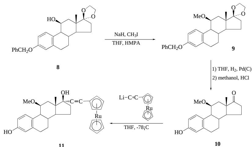
Scheme 3. Synthesis of 17\alpha -(ruthenocenylolethynyl)- 11\beta -methoxyestra-1,3,5(10)-trien-3,17 \beta -diol ( 11 ).
